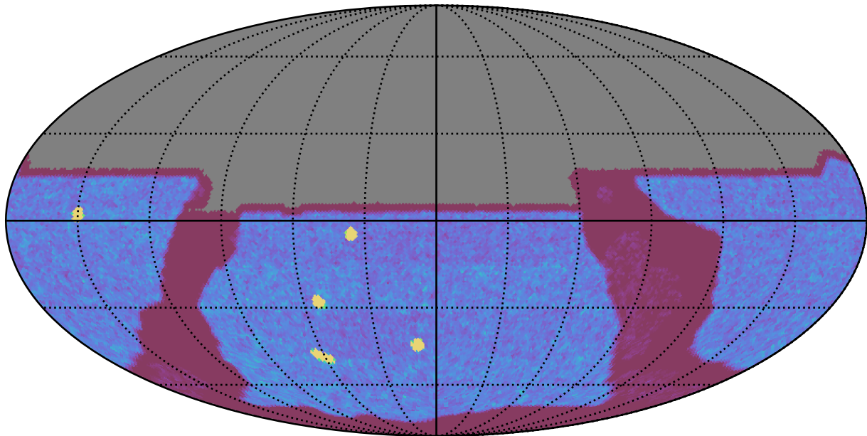
ddf_acor_sf30_lsf40_lsr10_v3.4_10yrs All sky y band: NVisits
