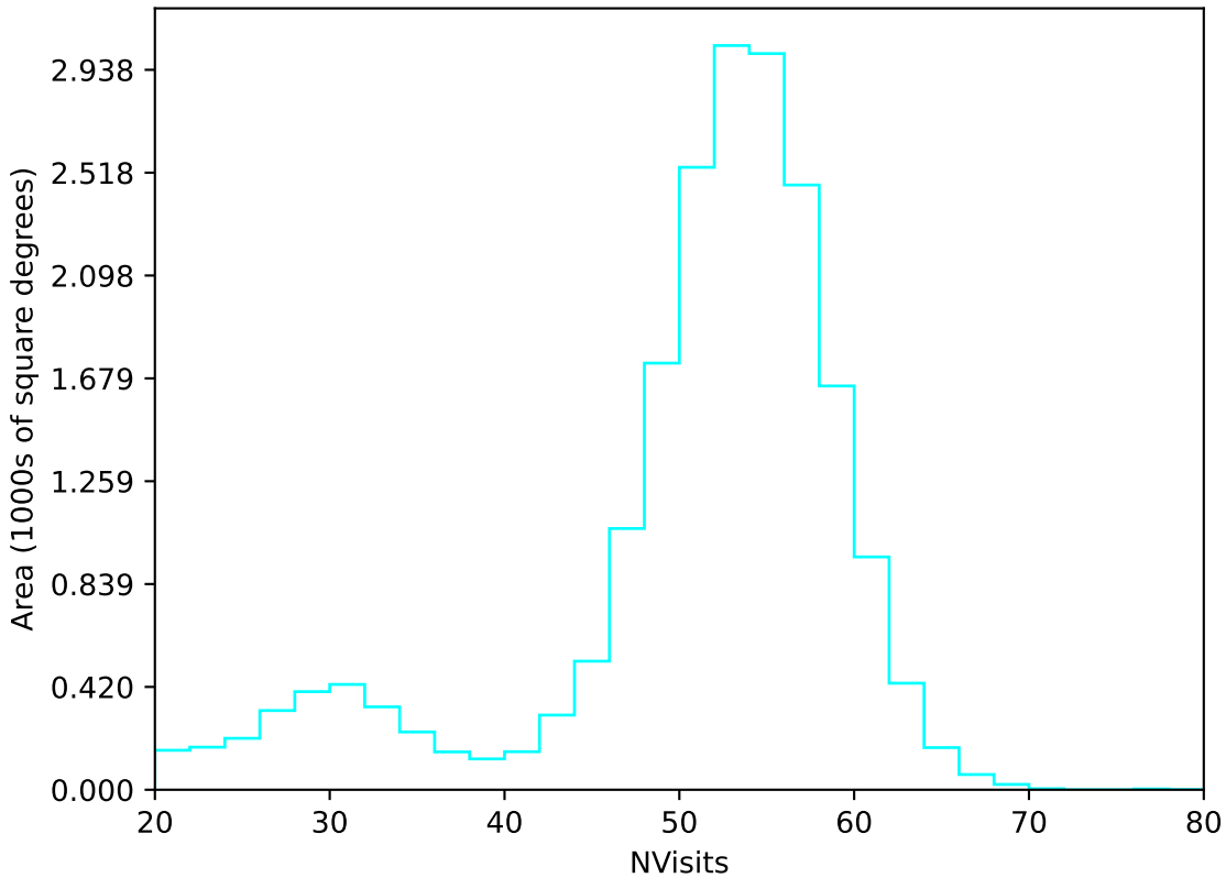
ddf_acor_sf30_lsf40_lsr10_v3.4_10yrs All sky u band: NVisits
