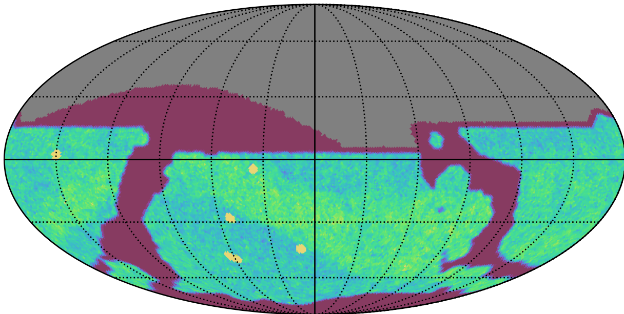
ddf_acor_sf30_lsf40_lsr10_v3.4_10yrs All sky i band: NVisits
