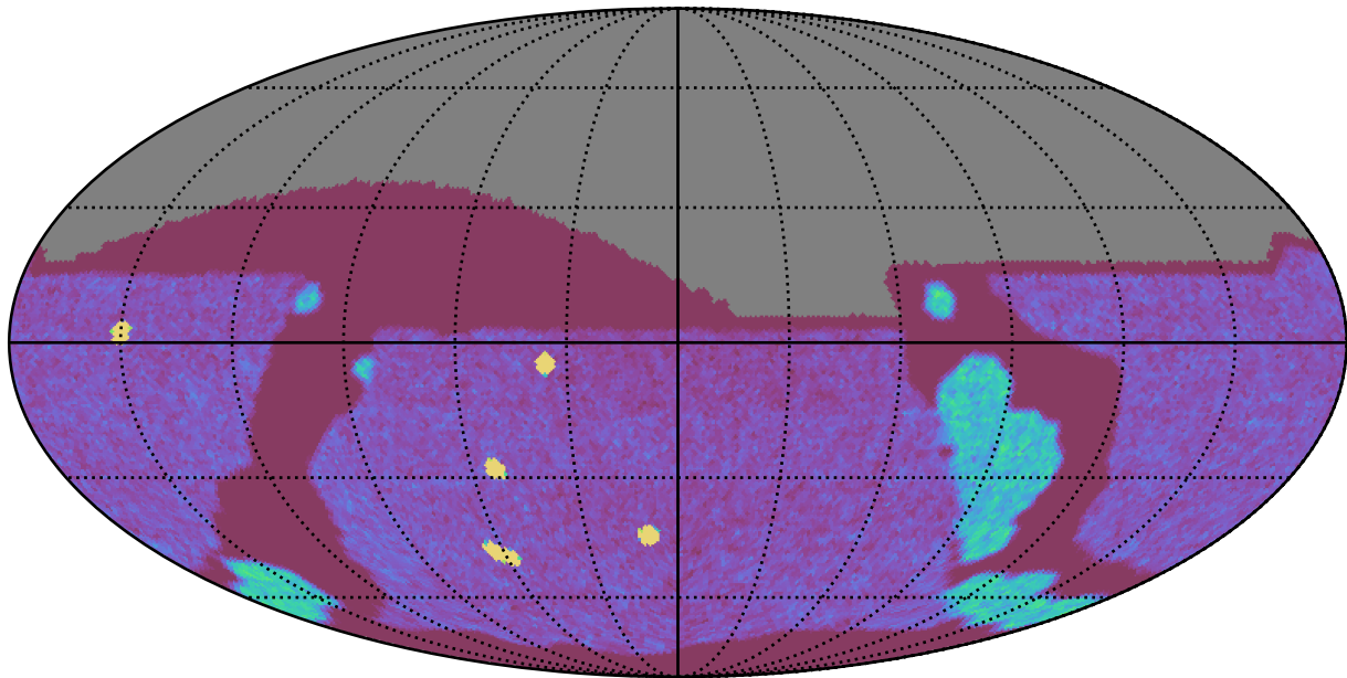
ddf_acor_sf30_lsf40_lsr10_v3.4_10yrs All sky g band: NVisits
