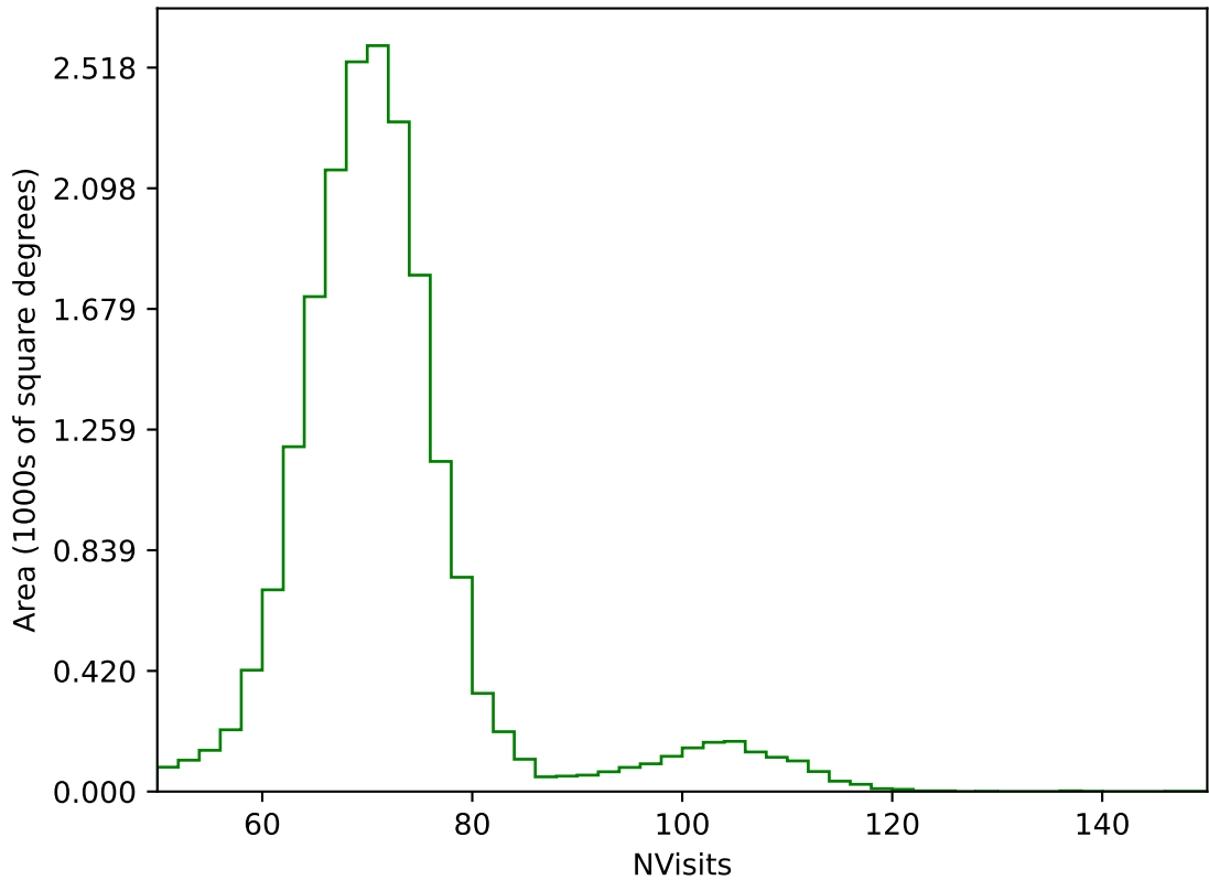
ddf_acor_sf30_lsf40_lsr10_v3.4_10yrs All sky g band: NVisits
