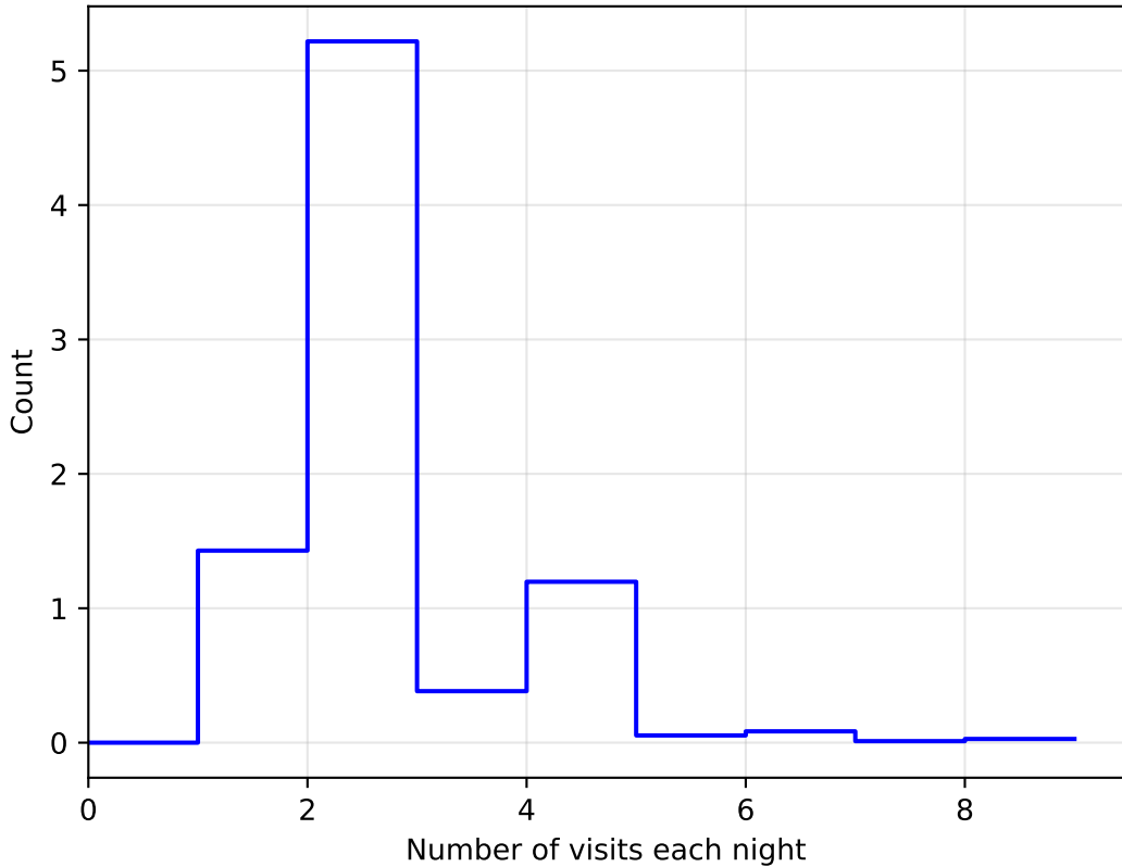
ddf_acor_sf30_lsf40_lsr10_v3.4_10yrs WFD: NVisitsPerNight 1e6
