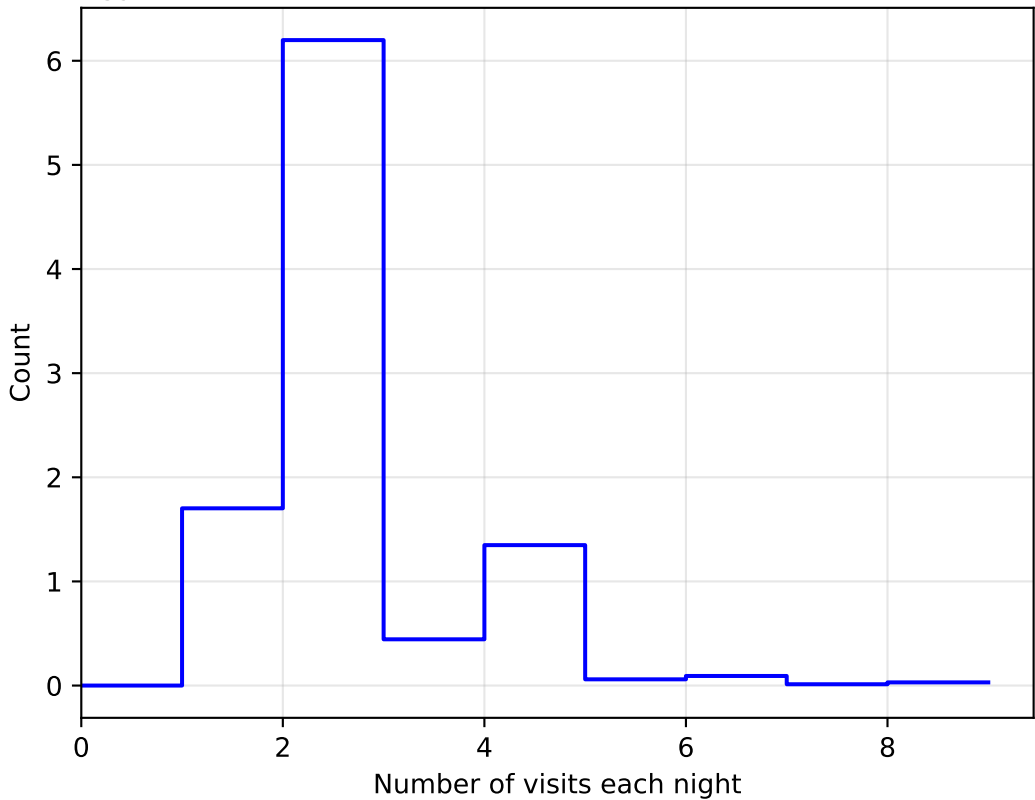
ddf_acor_sf30_lsf40_lsr10_v3.4_10yrs All sky: NVisitsPerNight 1e6
