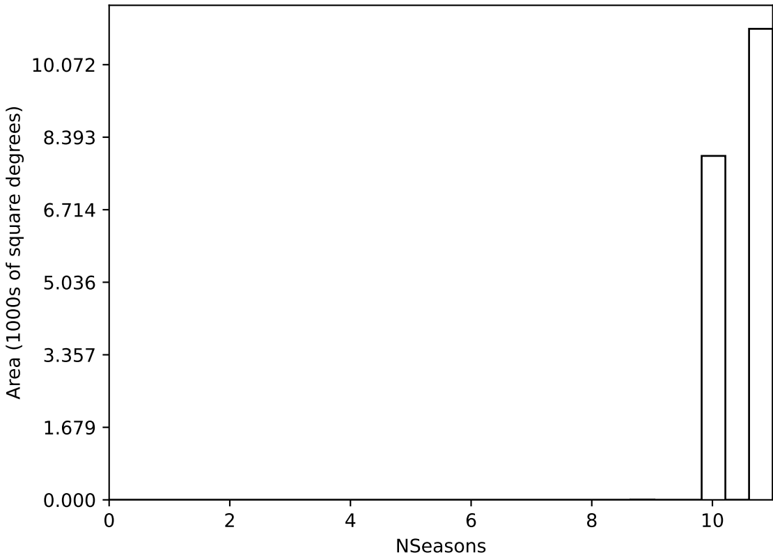
ddf_acor_sf30_lsf40_lsr10_v3.4_10yrs WFD all bands: NSeasons
