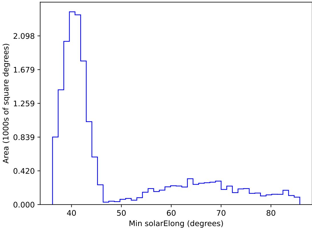
ddf_acor_sf30_lsf40_lsr10_v3.4_10yrs WFD z band: Min solarElong
