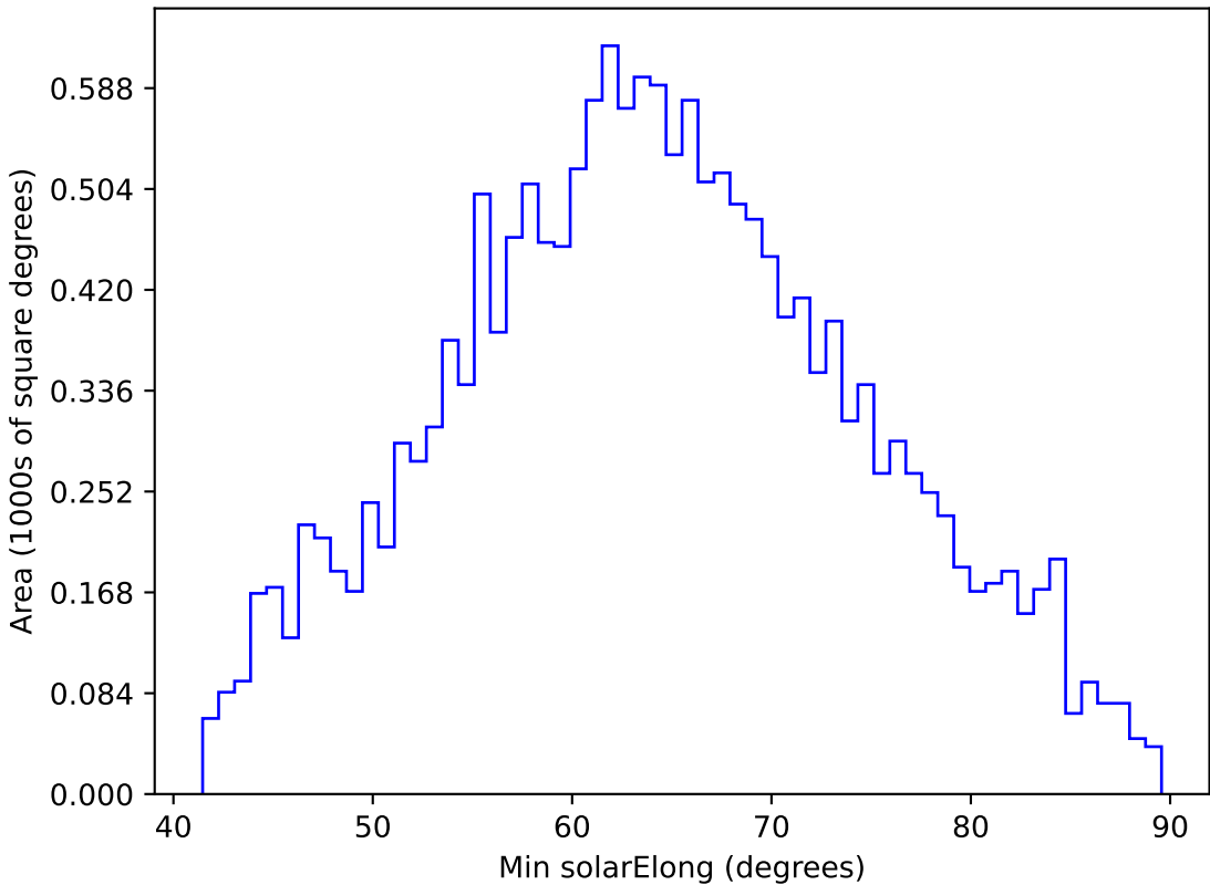
ddf_acor_sf30_lsf40_lsr10_v3.4_10yrs WFD y band: Min solarElong
