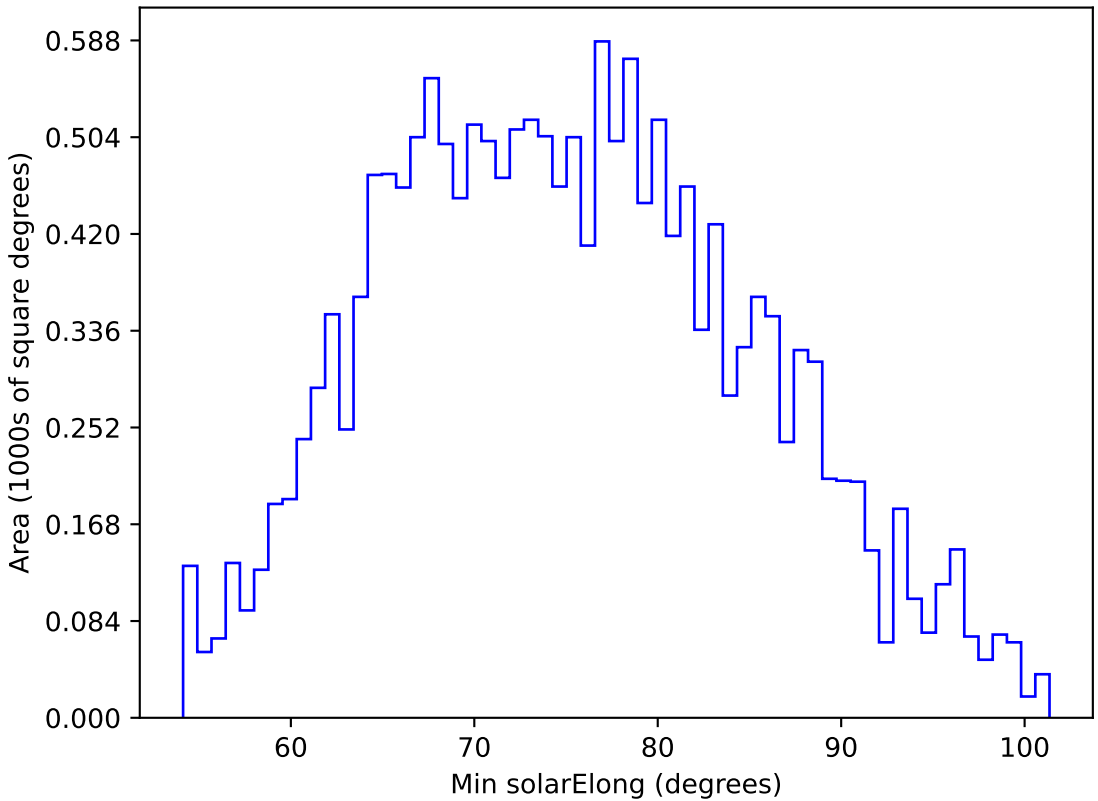
ddf_acor_sf30_lsf40_lsr10_v3.4_10yrs WFD u band: Min solarElong
