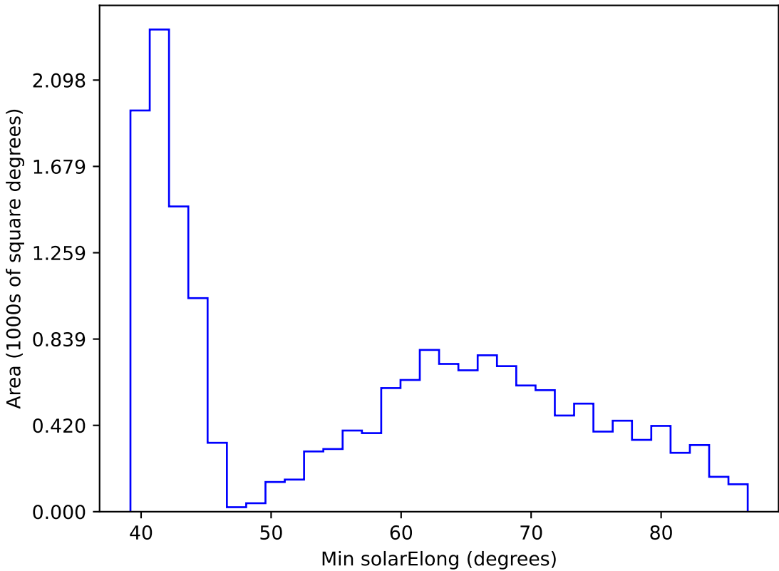
ddf_acor_sf30_lsf40_lsr10_v3.4_10yrs WFD r band: Min solarElong
