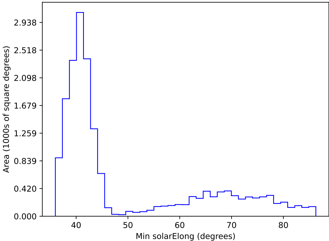
ddf_acor_sf30_lsf40_lsr10_v3.4_10yrs WFD i band: Min solarElong
