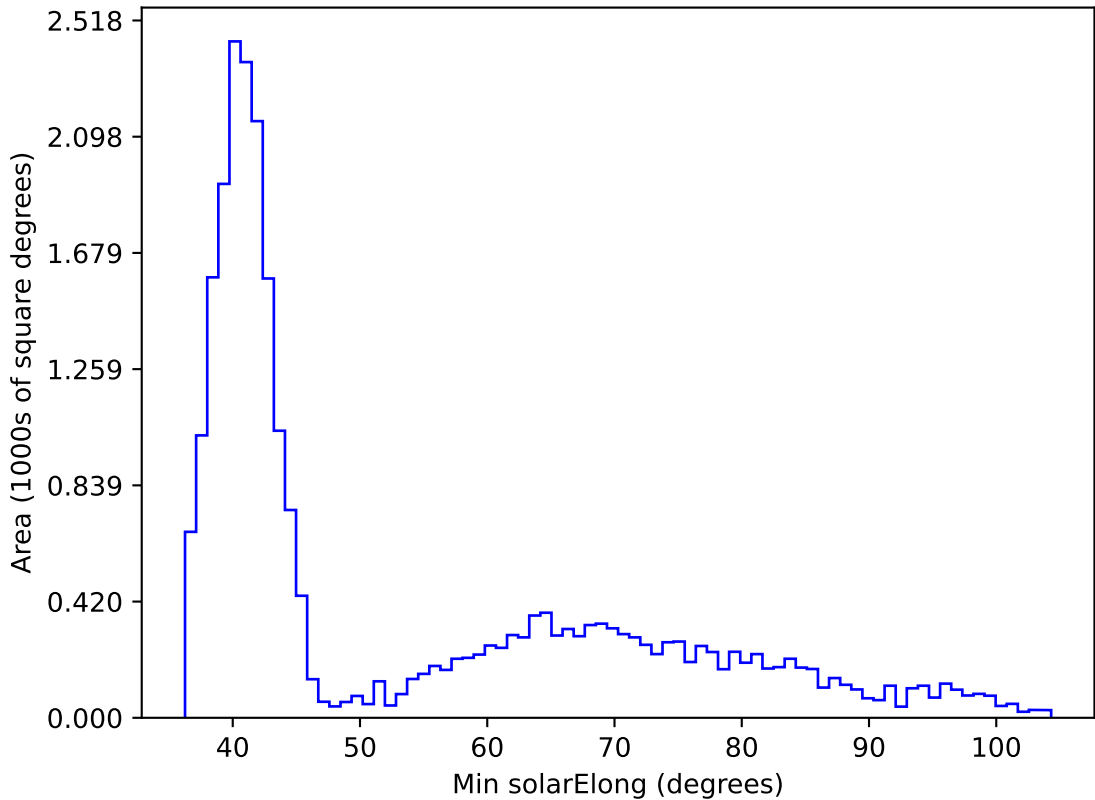
ddf_acor_sf30_lsf40_lsr10_v3.4_10yrs All sky z band: Min solarElong
