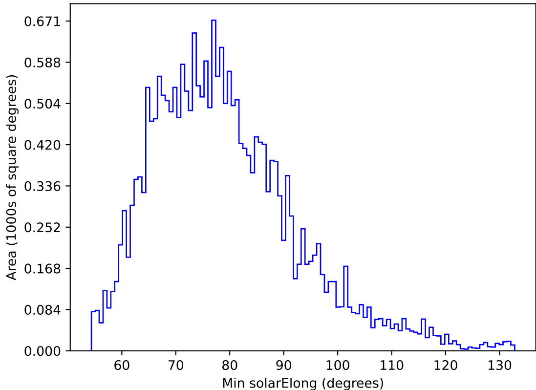
ddf_acor_sf30_lsf40_lsr10_v3.4_10yrs All sky u band: Min solarElong
