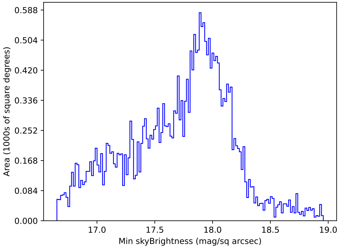
ddf_acor_sf30_lsf40_lsr10_v3.4_10yrs Yr 1 all bands: Min skyBrightness
