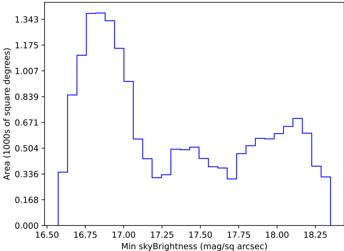
ddf_acor_sf30_lsf40_lsr10_v3.4_10yrs WFD z band: Min skyBrightness
