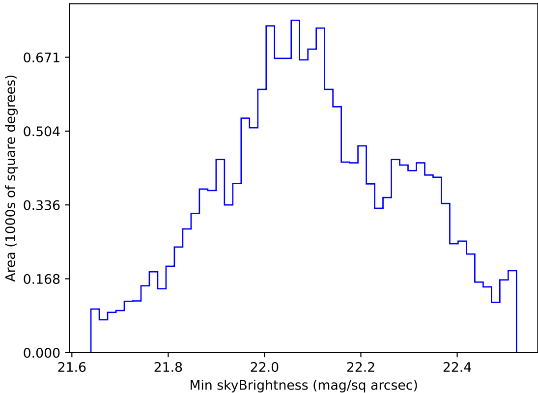
ddf_acor_sf30_lsf40_lsr10_v3.4_10yrs WFD u band: Min skyBrightness
