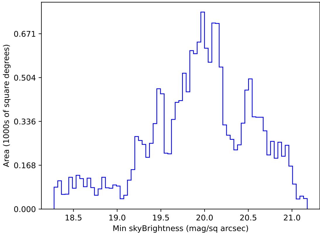
ddf_acor_sf30_lsf40_lsr10_v3.4_10yrs WFD g band: Min skyBrightness
