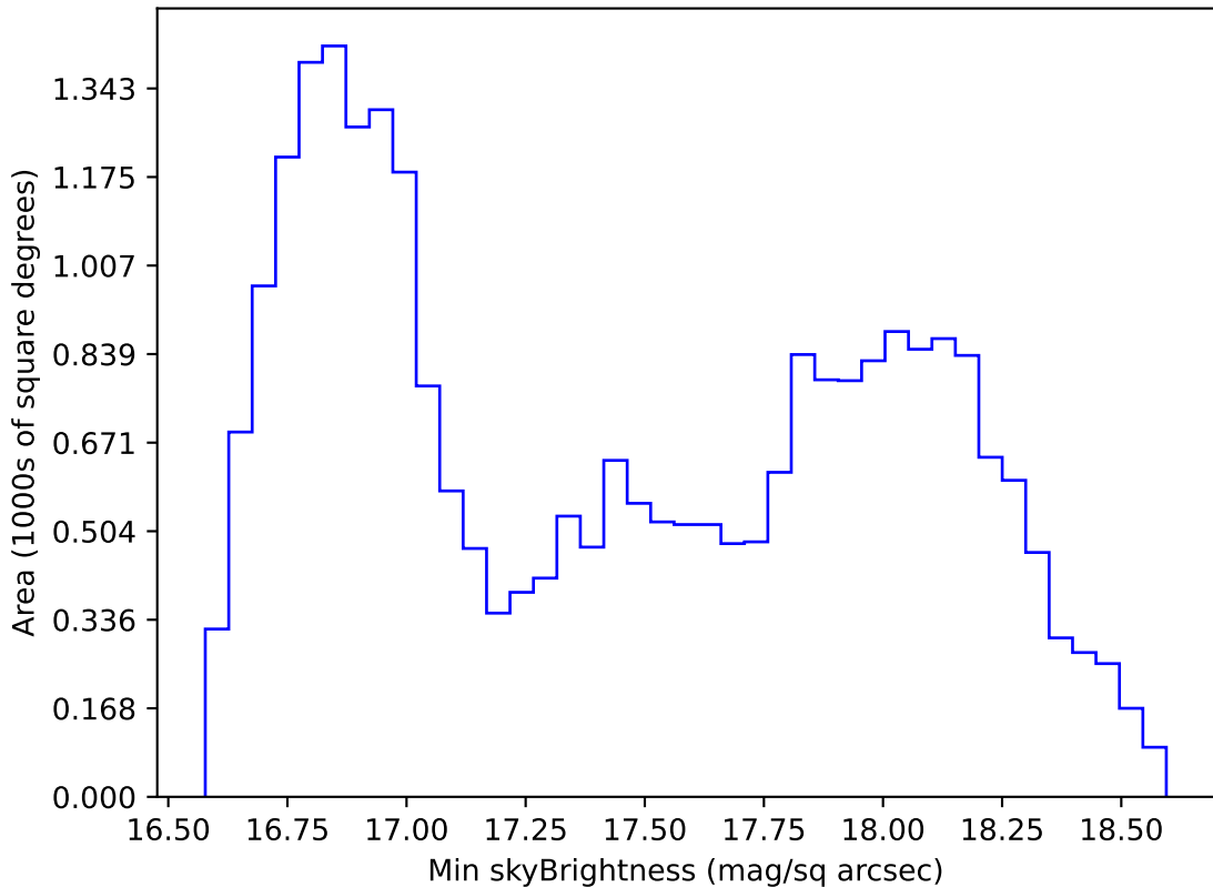
ddf_acor_sf30_lsf40_lsr10_v3.4_10yrs All sky z band: Min skyBrightness
