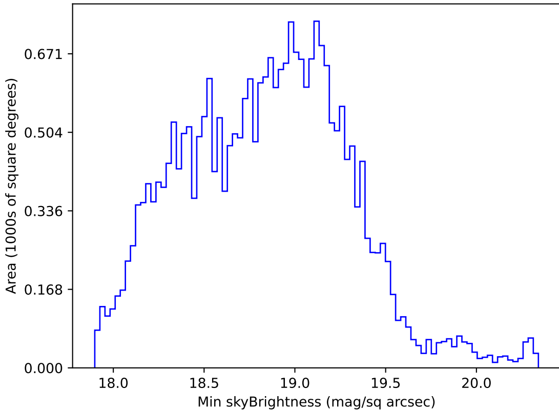
ddf_acor_sf30_lsf40_lsr10_v3.4_10yrs All sky r band: Min skyBrightness
