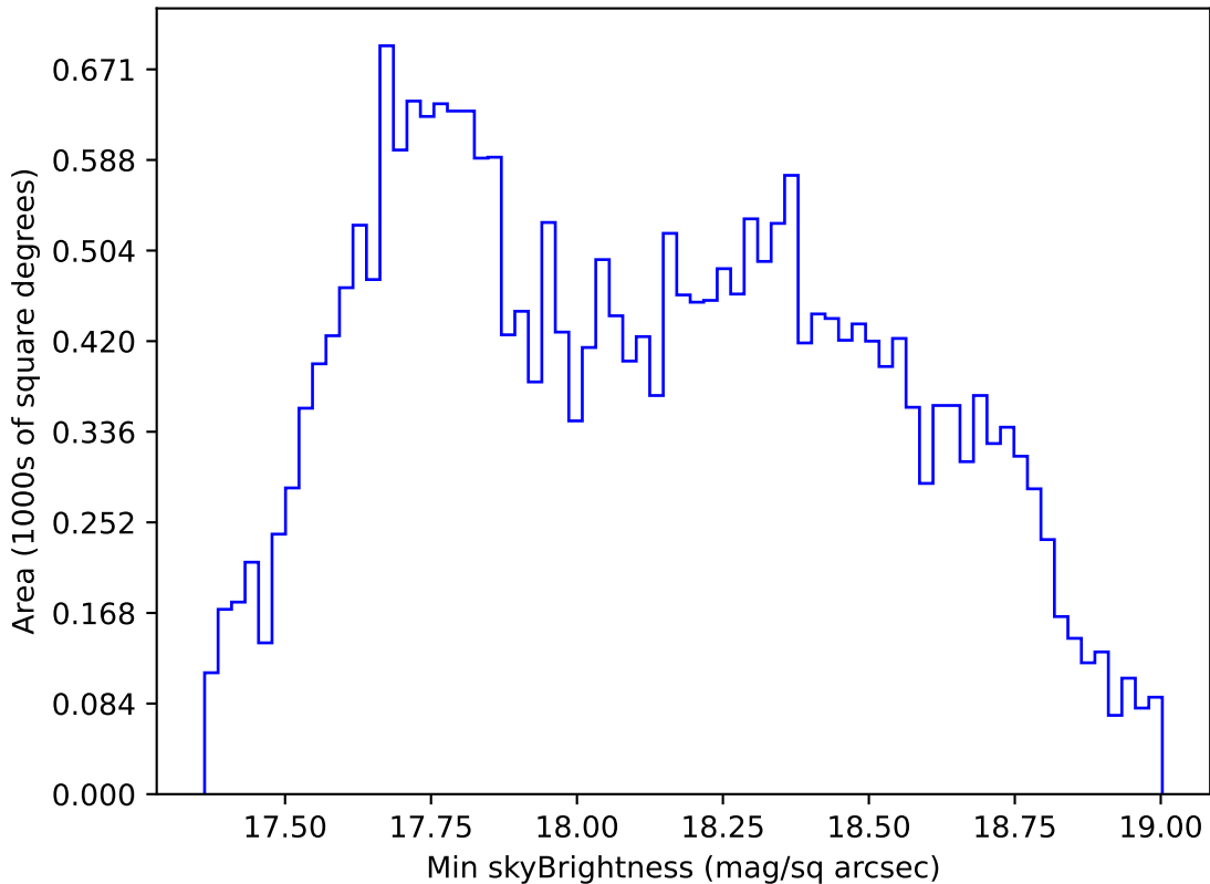
ddf_acor_sf30_lsf40_lsr10_v3.4_10yrs All sky i band: Min skyBrightness
