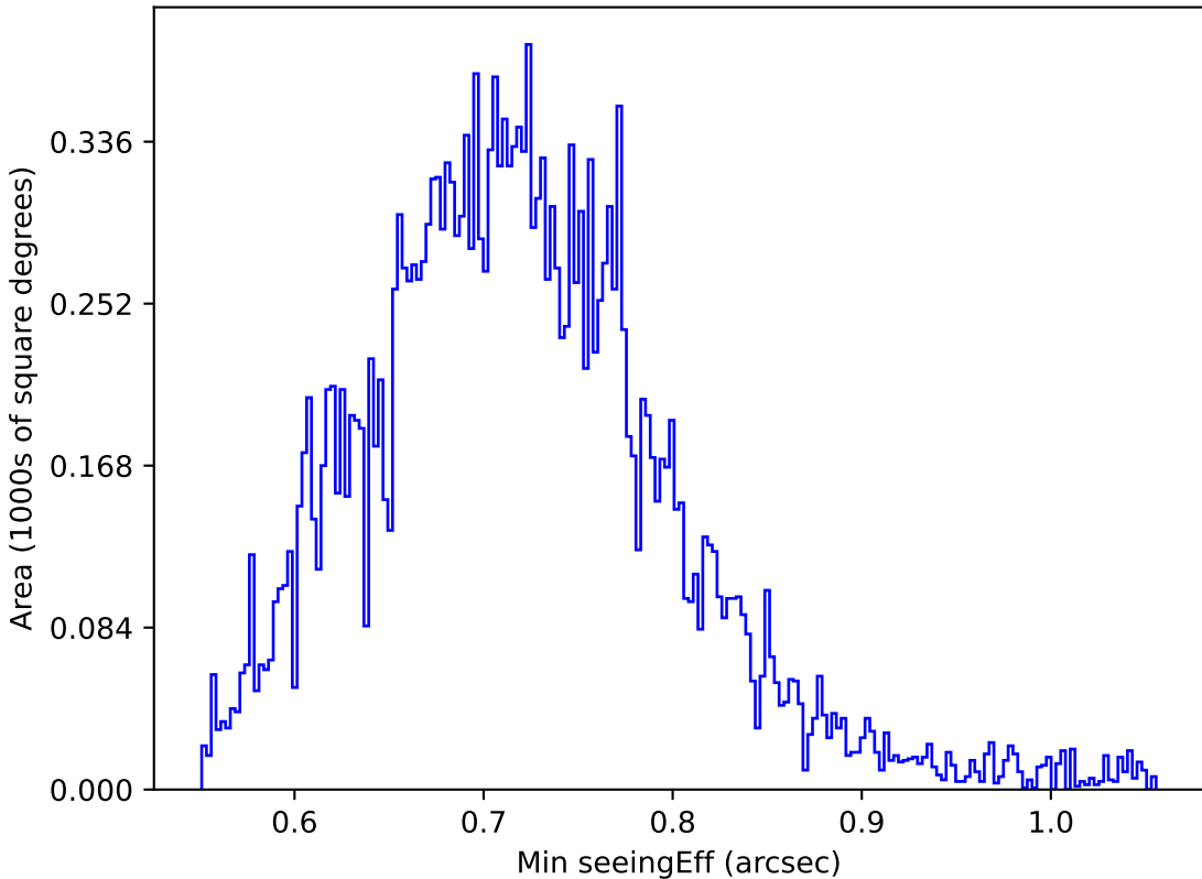
ddf_acor_sf30_lsf40_lsr10_v3.4_10yrs Yr 1 y band: Min seeingEff
