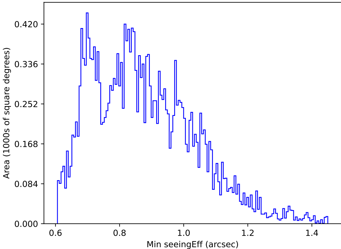
ddf_acor_sf30_lsf40_lsr10_v3.4_10yrs Yr 1 u band: Min seeingEff
