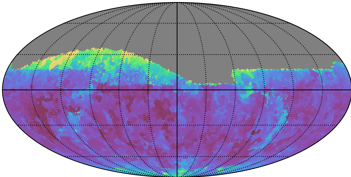
ddf_acor_sf30_lsf40_lsr10_v3.4_10yrs Yr 1 i band: Min seeingEff
