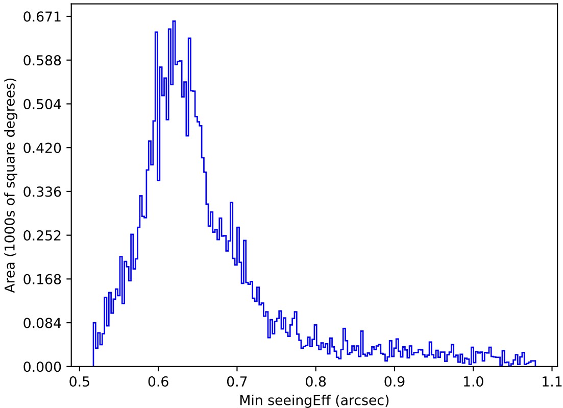
ddf_acor_sf30_lsf40_lsr10_v3.4_10yrs Yr 1 all bands: Min seeingEff
