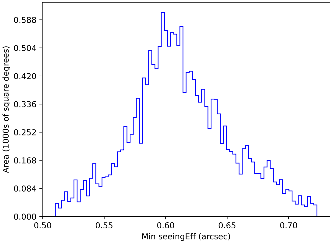
ddf_acor_sf30_lsf40_lsr10_v3.4_10yrs WFD z band: Min seeingEff
