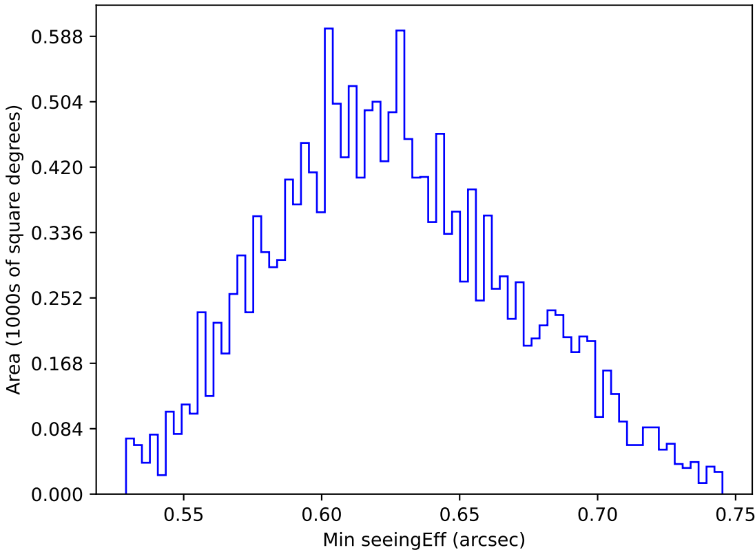
ddf_acor_sf30_lsf40_lsr10_v3.4_10yrs WFD y band: Min seeingEff
