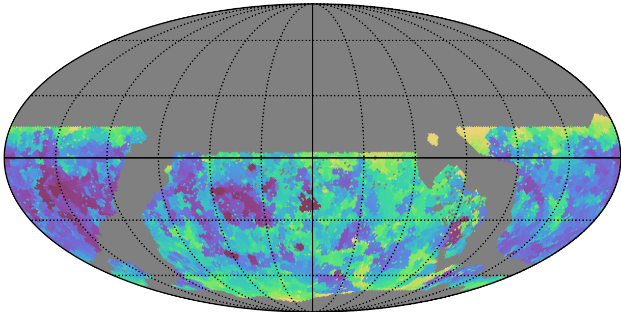
ddf_acor_sf30_lsf40_lsr10_v3.4_10yrs WFD u band: Min seeingEff
