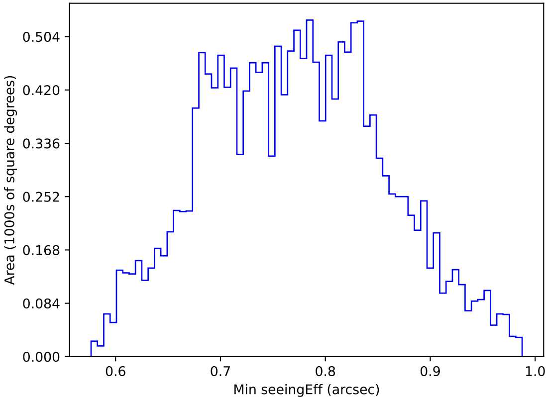
ddf_acor_sf30_lsf40_lsr10_v3.4_10yrs WFD u band: Min seeingEff
