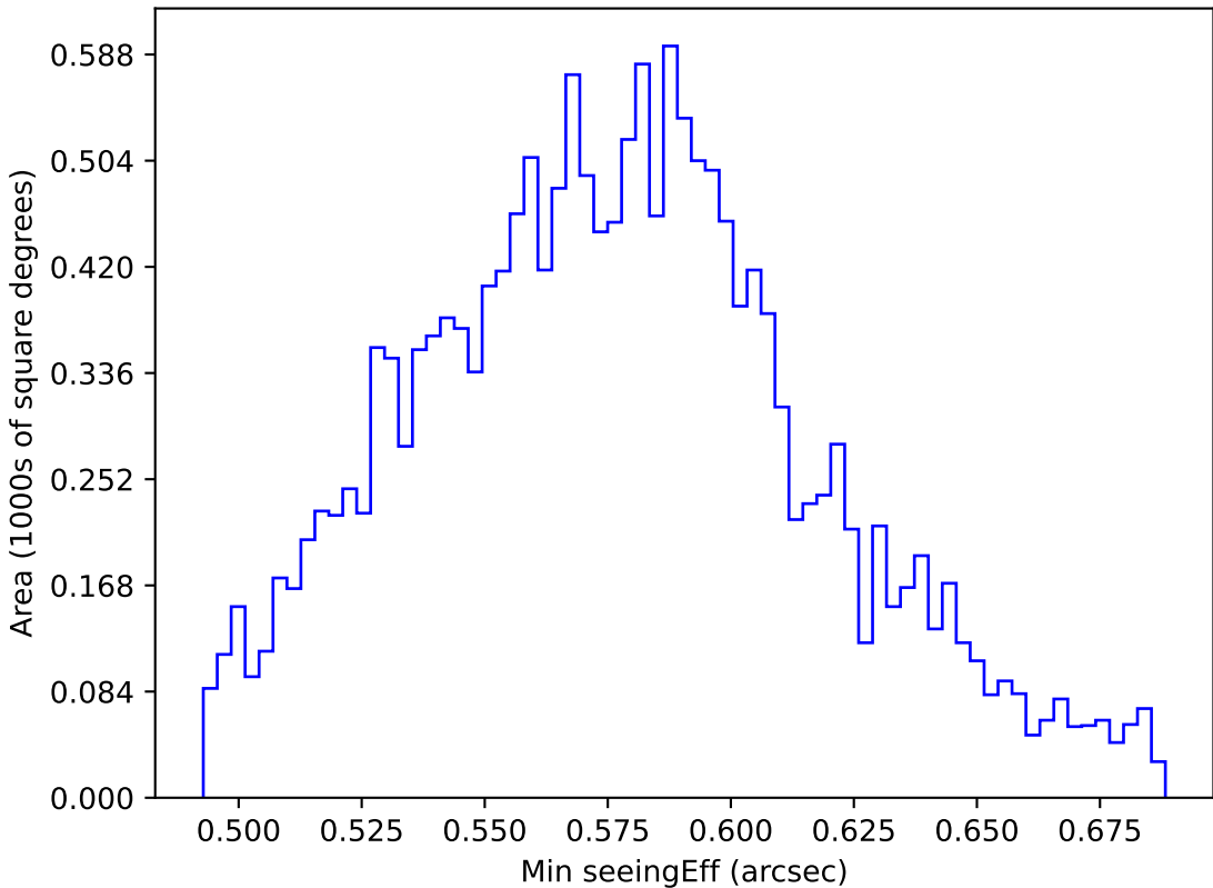
ddf_acor_sf30_lsf40_lsr10_v3.4_10yrs WFD all bands: Min seeingEff
