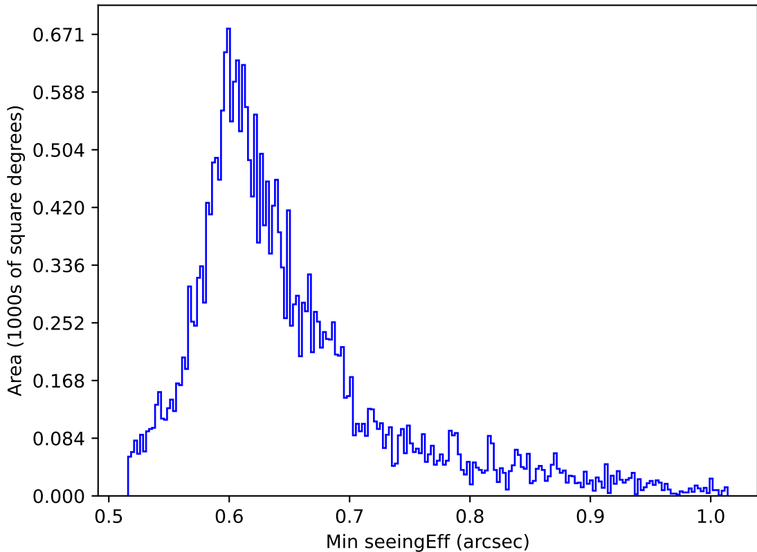
ddf_acor_sf30_lsf40_lsr10_v3.4_10yrs All sky z band: Min seeingEff
