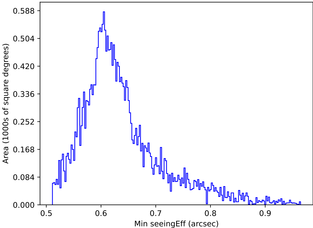
ddf_acor_sf30_lsf40_lsr10_v3.4_10yrs All sky i band: Min seeingEff
