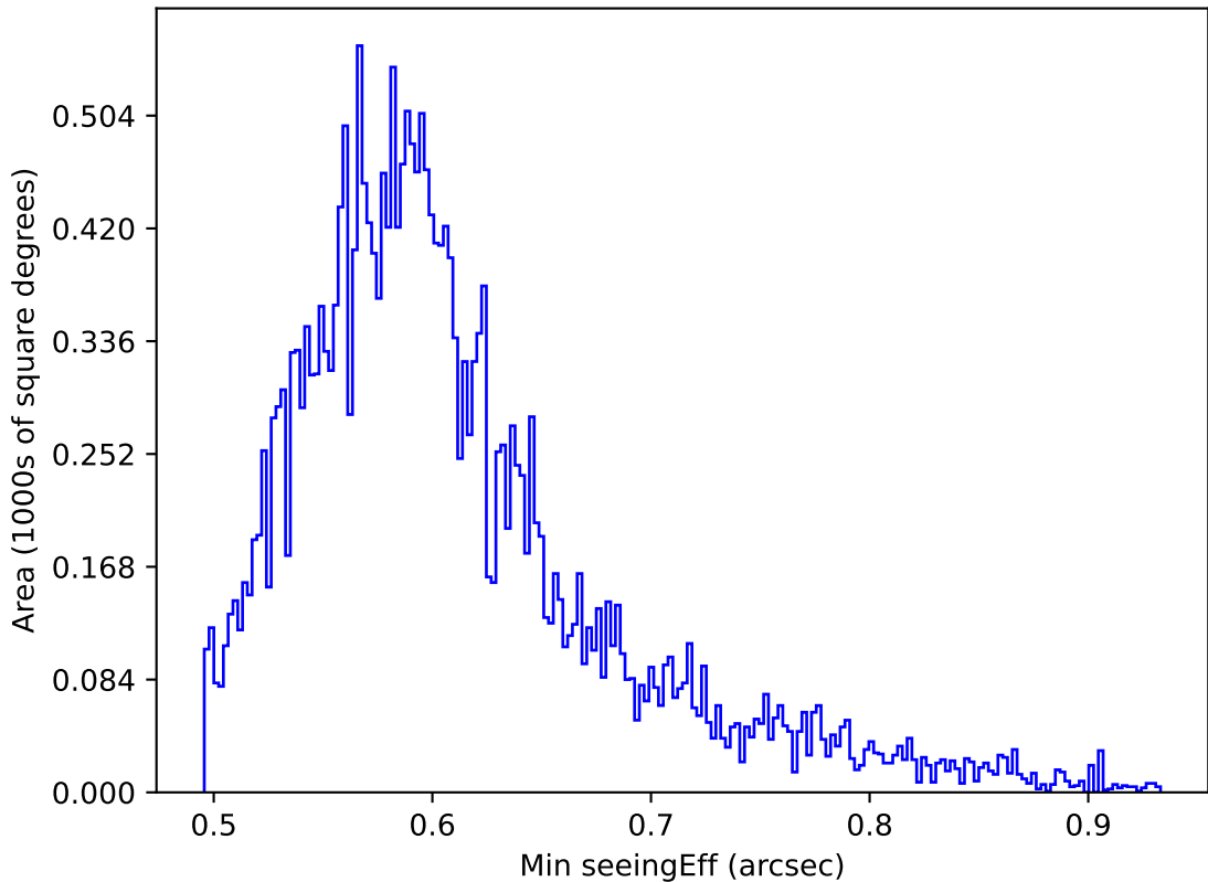
ddf_acor_sf30_lsf40_lsr10_v3.4_10yrs All sky all bands: Min seeingEff
