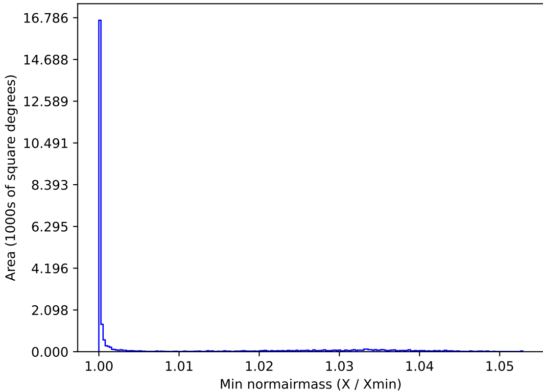
ddf_acor_sf30_lsf40_lsr10_v3.4_10yrs All sky g band: Min normairmass
