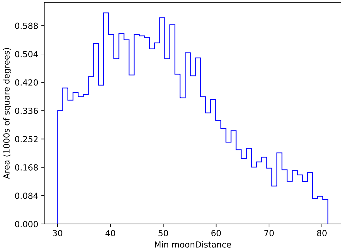
ddf_acor_sf30_lsf40_lsr10_v3.4_10yrs WFD u band: Min moonDistance
