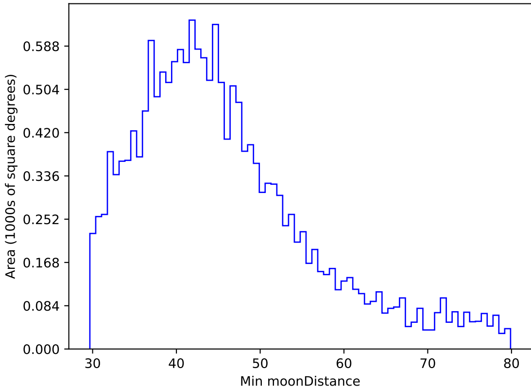
ddf_acor_sf30_lsf40_lsr10_v3.4_10yrs WFD g band: Min moonDistance
