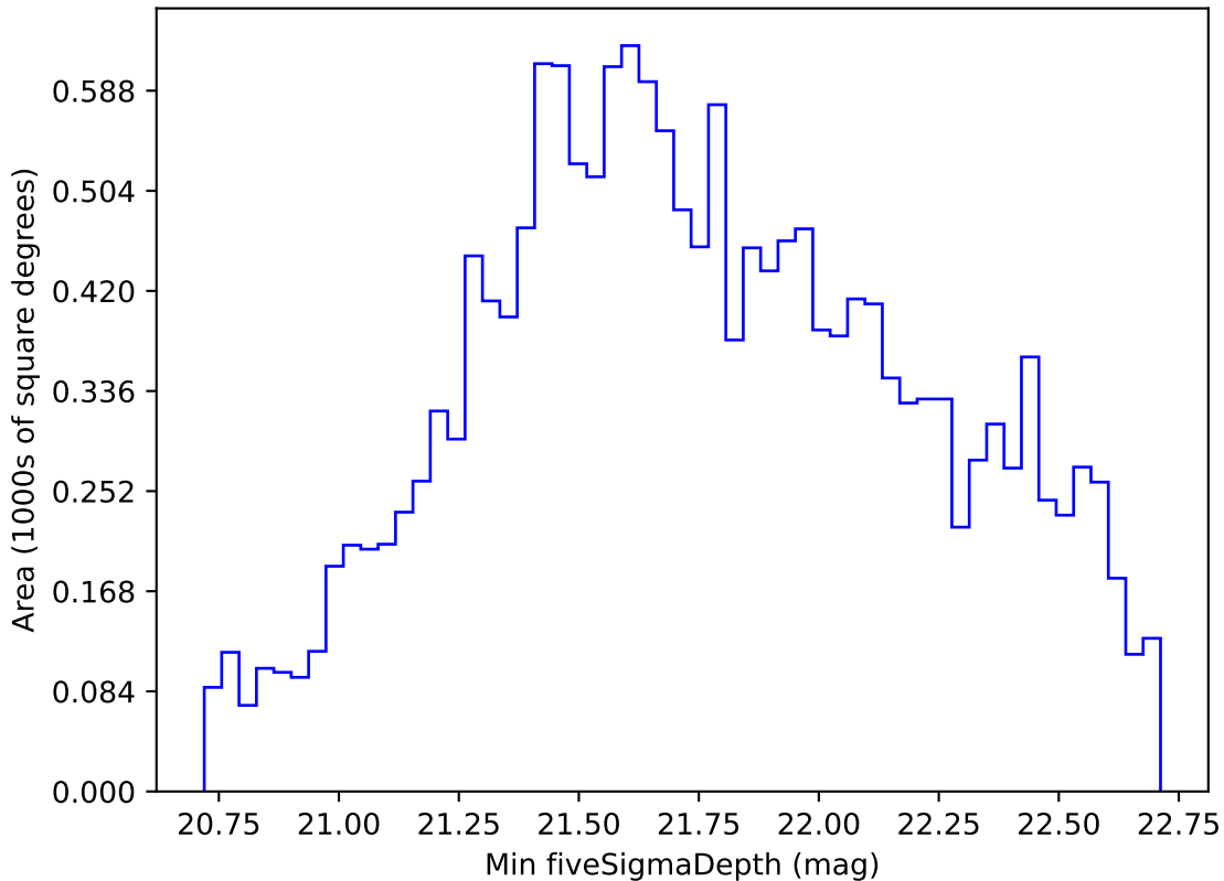
ddf_acor_sf30_lsf40_lsr10_v3.4_10yrs WFD i band: Min fiveSigmaDepth
