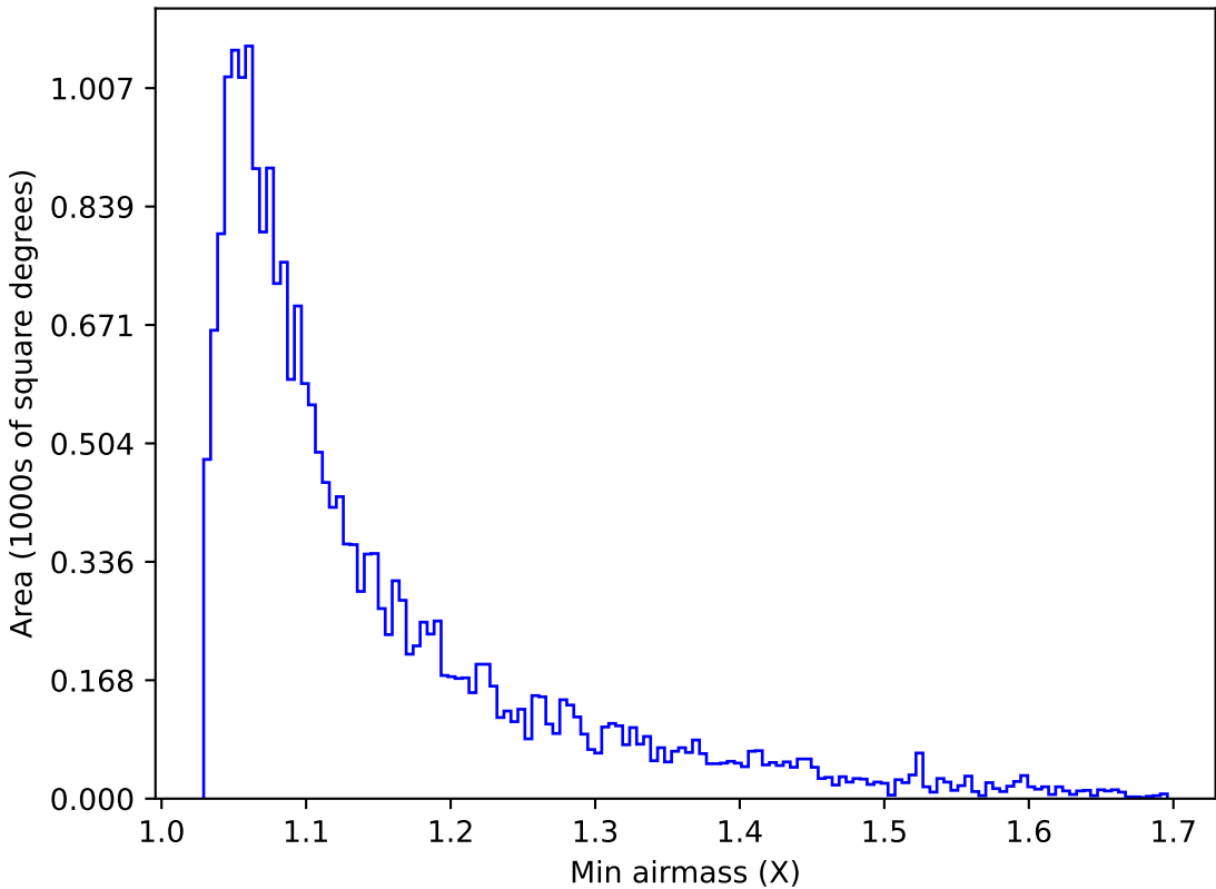
ddf_acor_sf30_lsf40_lsr10_v3.4_10yrs Yr 1 u band: Min airmass
