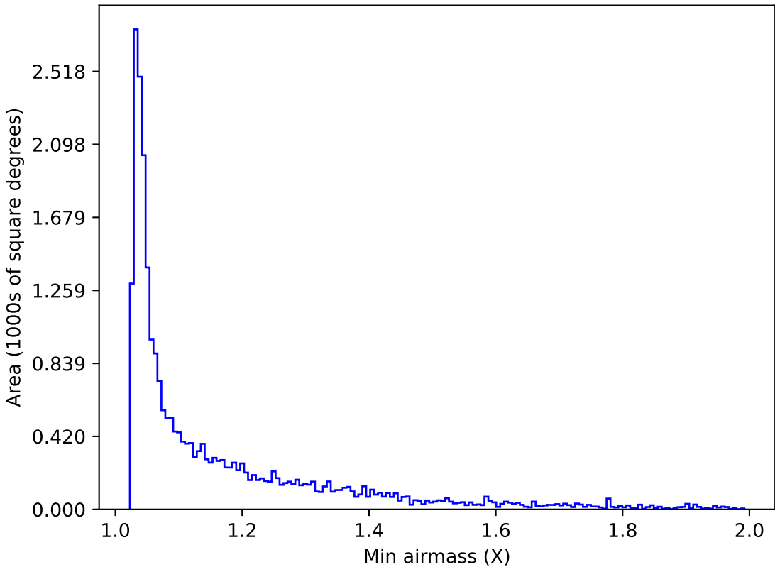
ddf_acor_sf30_lsf40_lsr10_v3.4_10yrs Yr 1 r band: Min airmass
