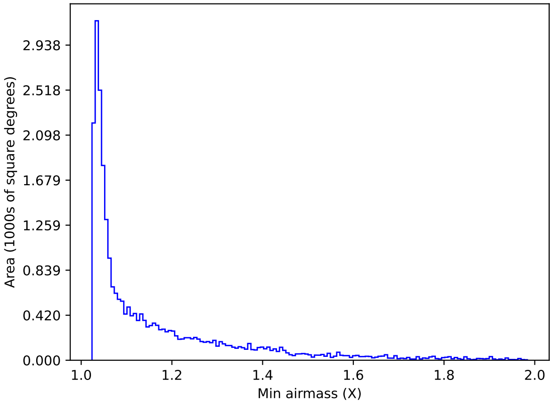
ddf_acor_sf30_lsf40_lsr10_v3.4_10yrs Yr 1 i band: Min airmass
