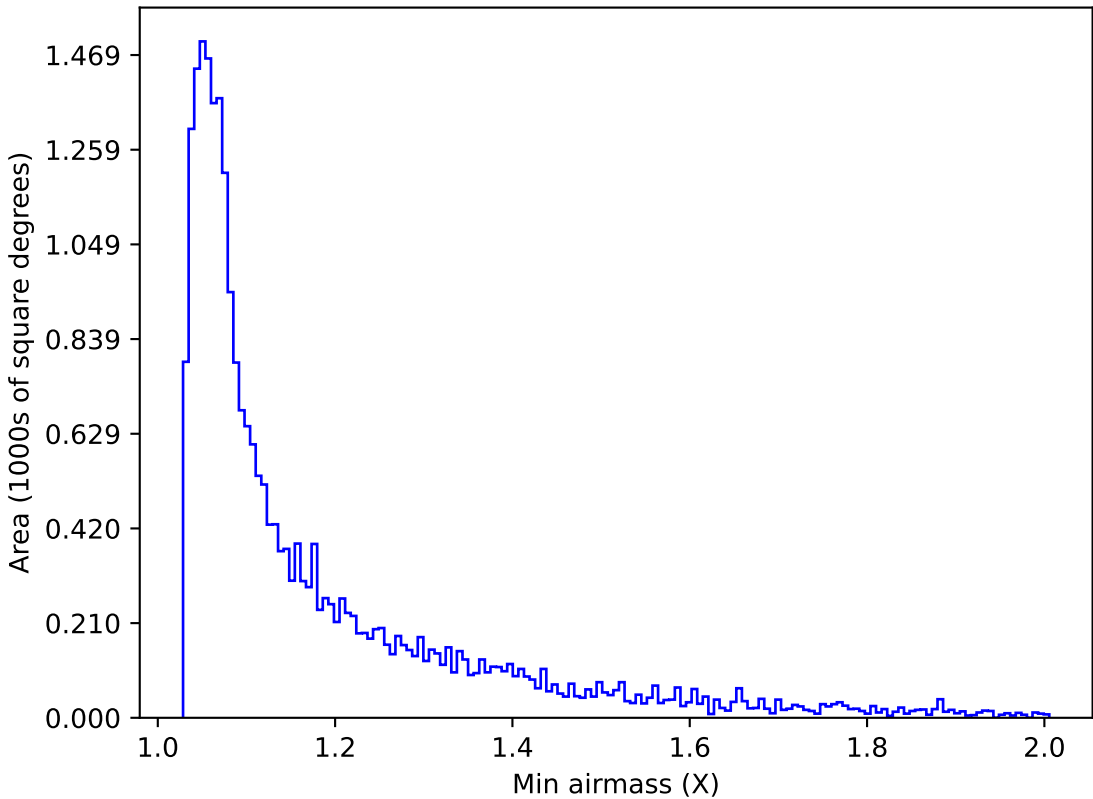
ddf_acor_sf30_lsf40_lsr10_v3.4_10yrs Yr 1 g band: Min airmass
