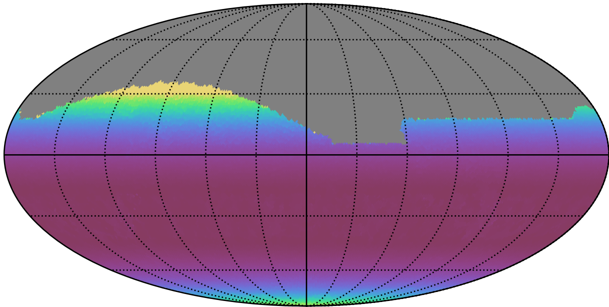
ddf_acor_sf30_lsf40_lsr10_v3.4_10yrs Yr 1 all bands: Min airmass
