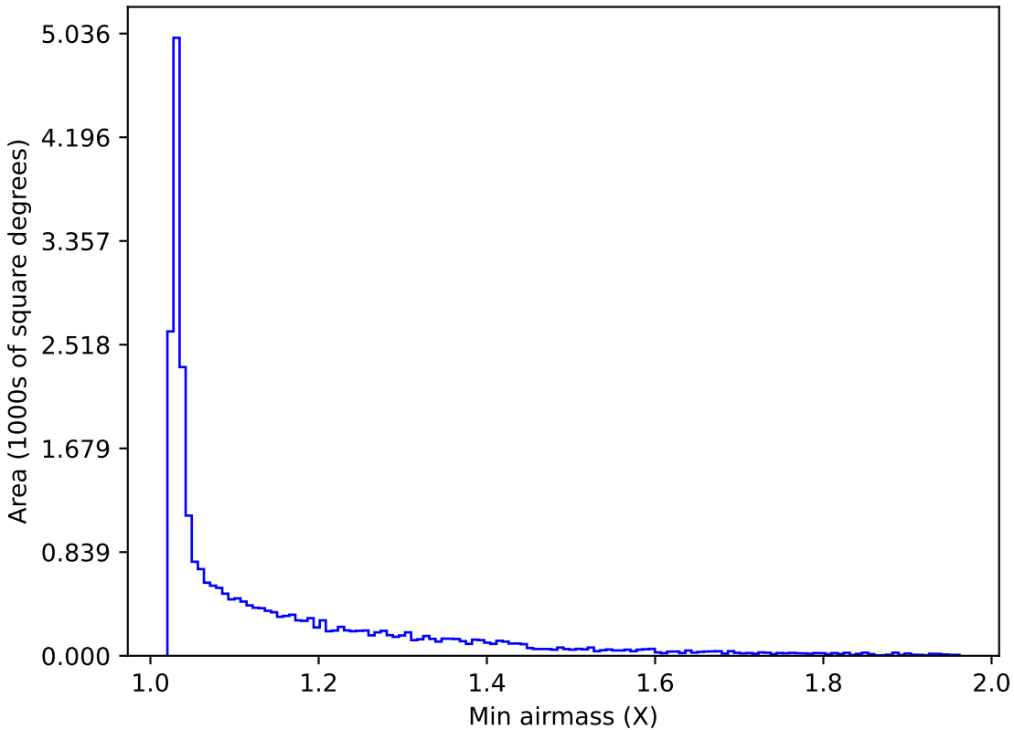
ddf_acor_sf30_lsf40_lsr10_v3.4_10yrs Yr 1 all bands: Min airmass
