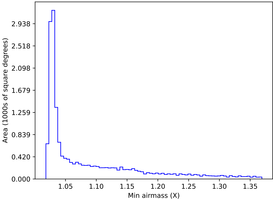
ddf_acor_sf30_lsf40_lsr10_v3.4_10yrs WFD z band: Min airmass
