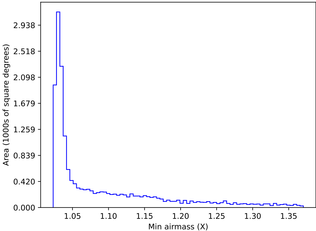
ddf_acor_sf30_lsf40_lsr10_v3.4_10yrs WFD y band: Min airmass
