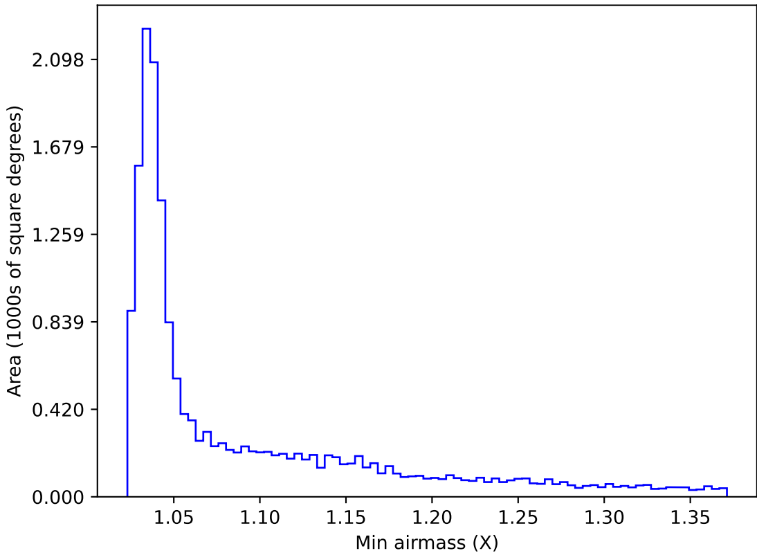
ddf_acor_sf30_lsf40_lsr10_v3.4_10yrs WFD g band: Min airmass
