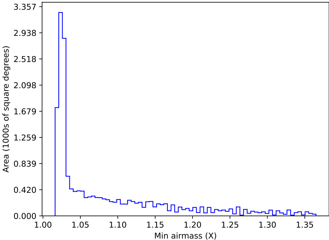
ddf_acor_sf30_lsf40_lsr10_v3.4_10yrs WFD all bands: Min airmass
