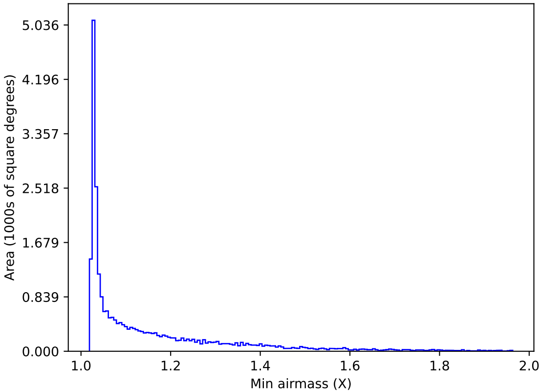
ddf_acor_sf30_lsf40_lsr10_v3.4_10yrs All sky z band: Min airmass
