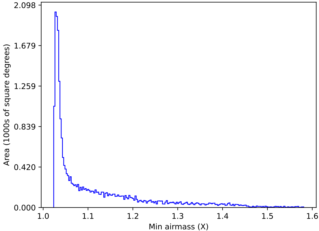
ddf_acor_sf30_lsf40_lsr10_v3.4_10yrs All sky y band: Min airmass
